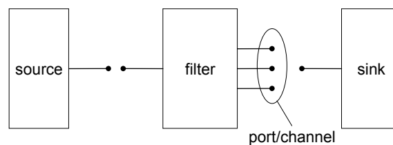
Figure 2: Media objects
